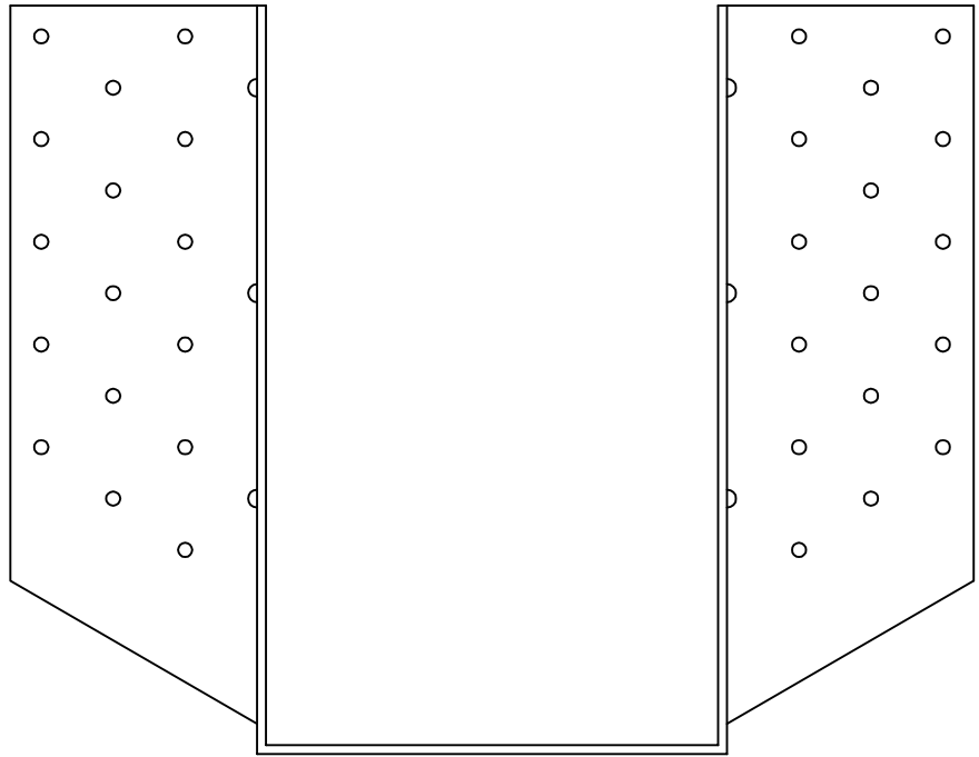
THD610 - FRONT VIEW
