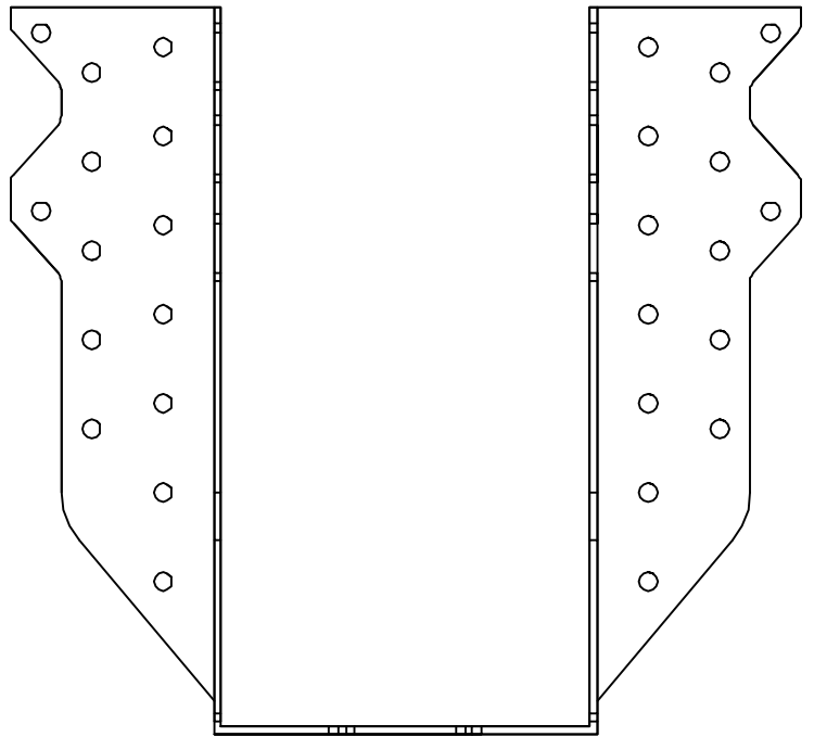
THD48 - FRONT VIEW
