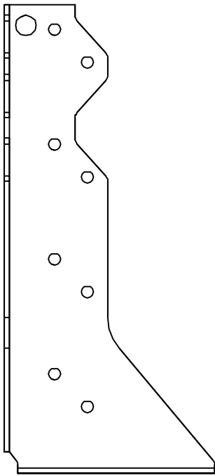
THD48 - SIDE VIEW
