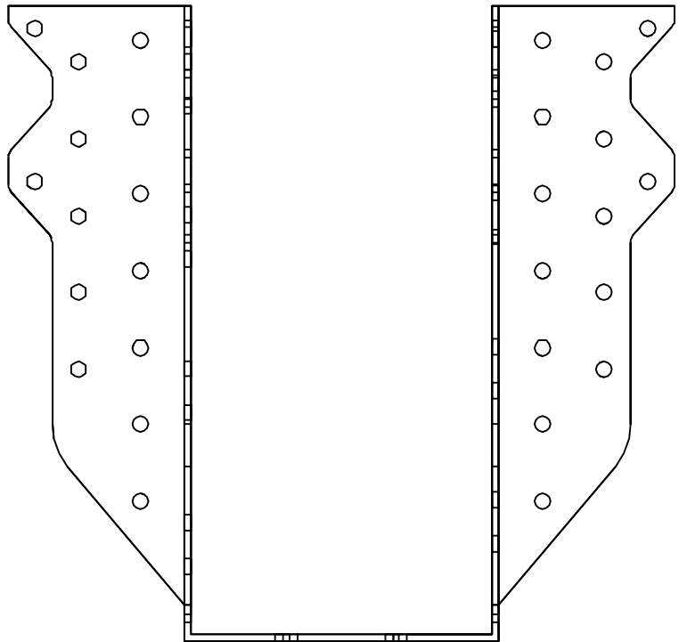
THD28-2 - FRONT VIEW
