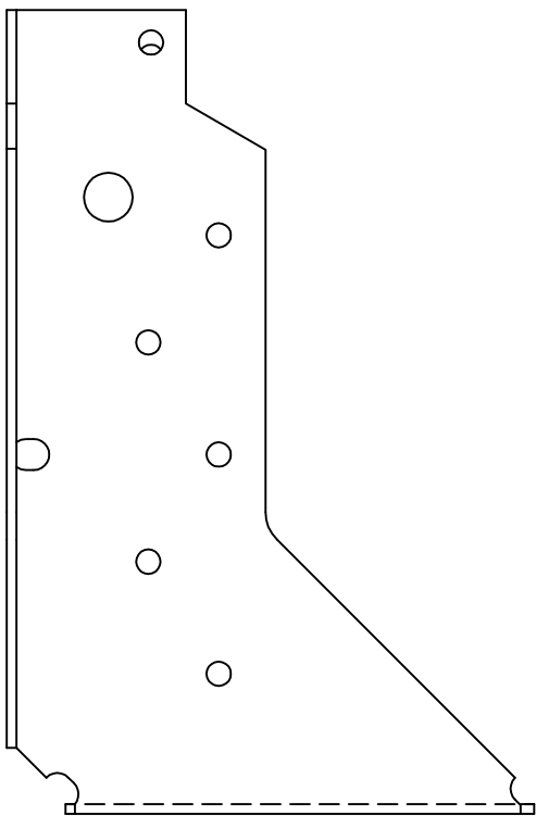
THD26 - SIDE VIEW
