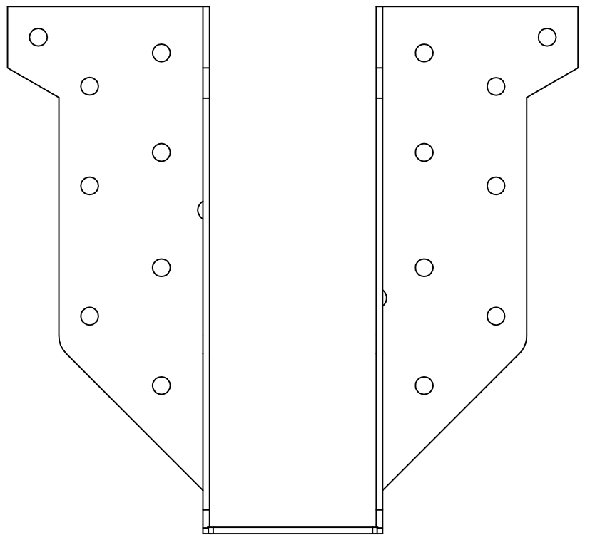
THD26 - FRONT VIEW
