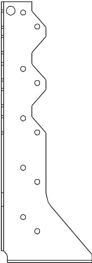
THD210-2 - SIDE VIEW
