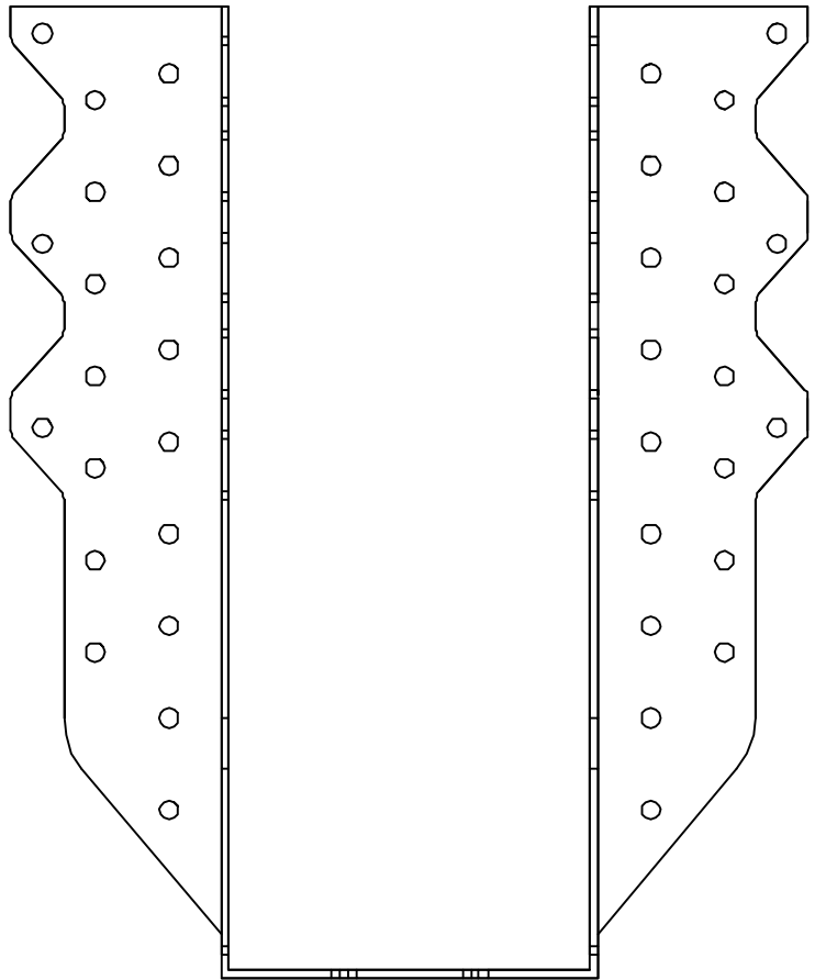
THD210-2 - FRONT VIEW
