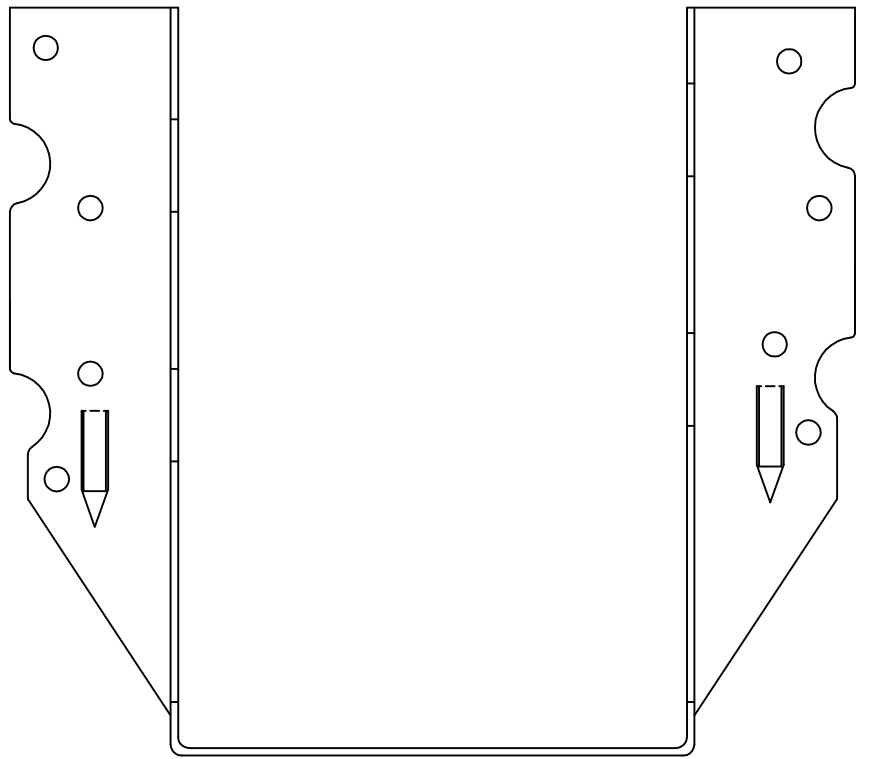
SUH46 - FRONT VIEW
