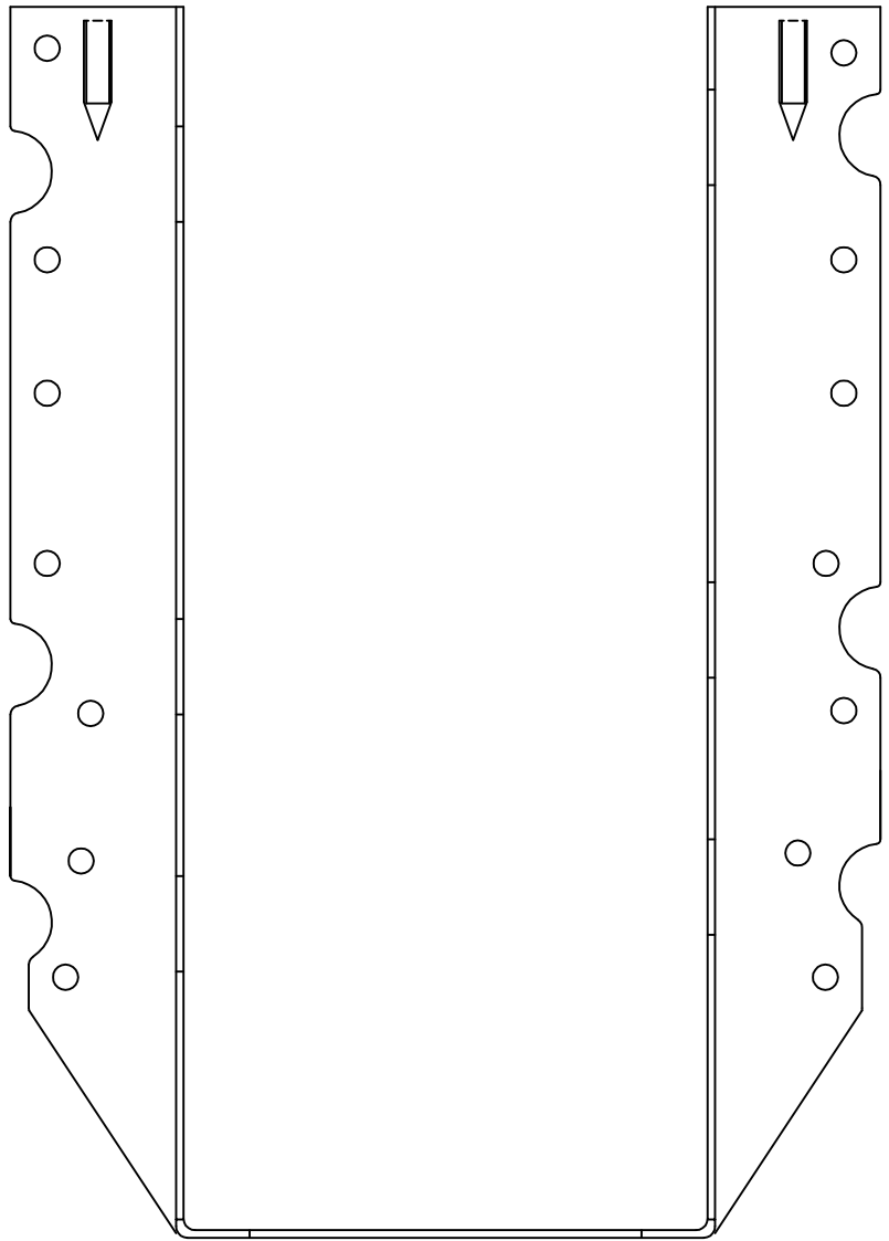
SUH410 - FRONT VIEW
