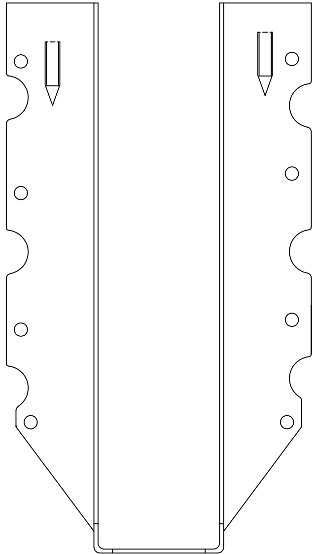
SUH28 - FRONT VIEW
