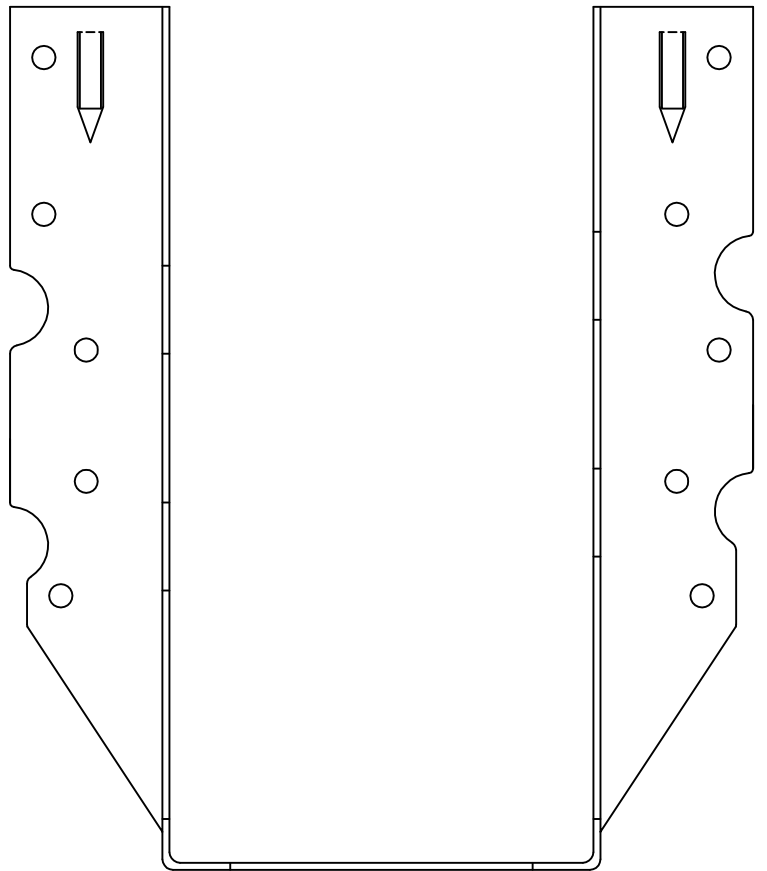
SUH28-2 - FRONT VIEW
