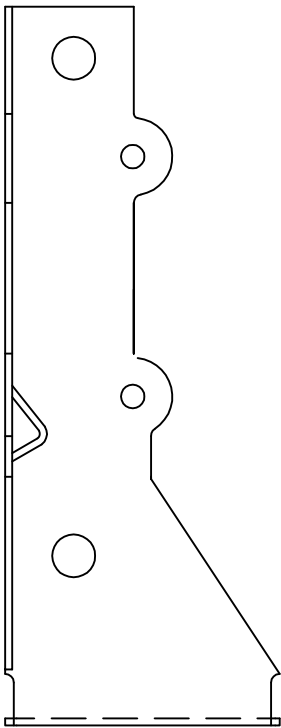
SUH26-2 SIDE VIEW
