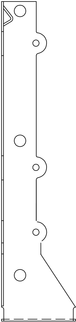
SUH210-2 - SIDE VIEW
