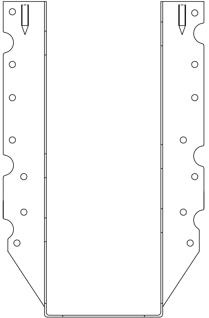
SUH210-2 - FRONT VIEW
