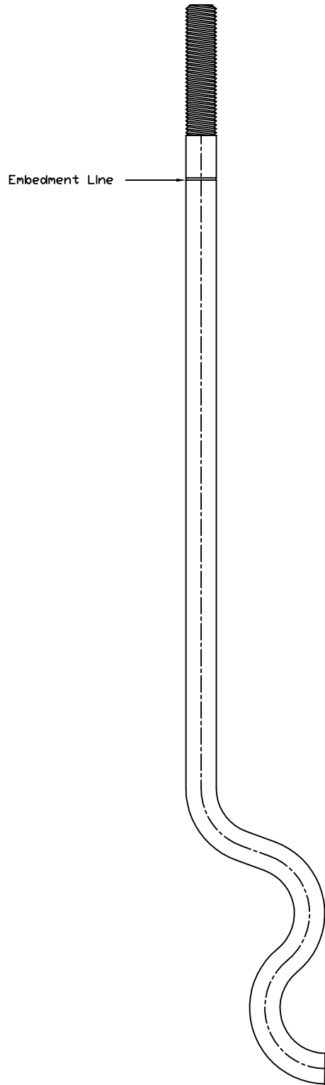
STB28 - SIDE VIEW
