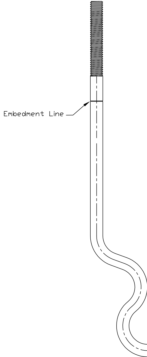
STB16 - SIDE VIEW
