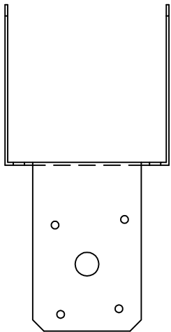
PCM46 - FRONT VIEW
