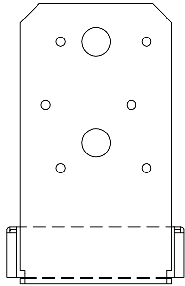
PAU44 - SIDE VIEW
