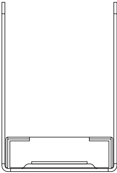
PAU44 - FRONT VIEW
