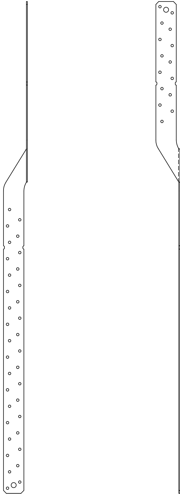
MTW30 - FRONT VIEW MTW30 - SIDE VIEW
