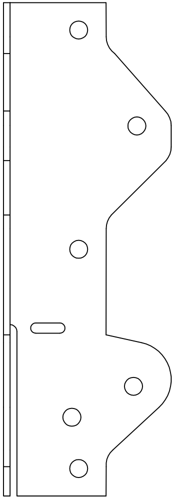
MPA1 - FRONT VIEW
