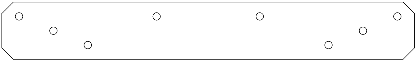
LSTA9 - FRONT VIEW
