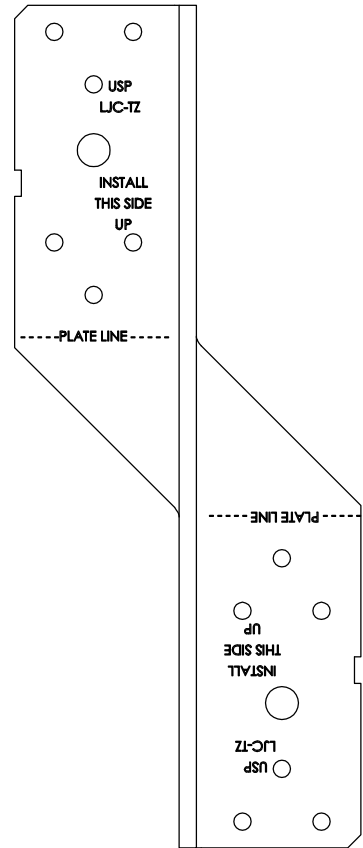
LJC-TZ-TOP-VIEW
