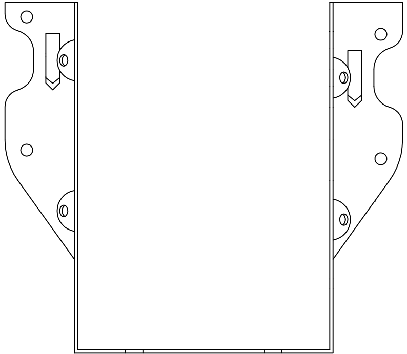
JUS46 - FRONT VIEW
