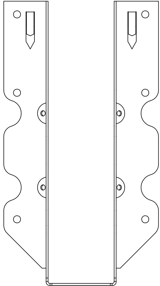
JUS28 - FRONT VIEW
