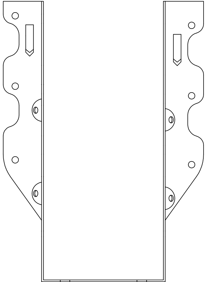
JUS28-2 - FRONT VIEW
