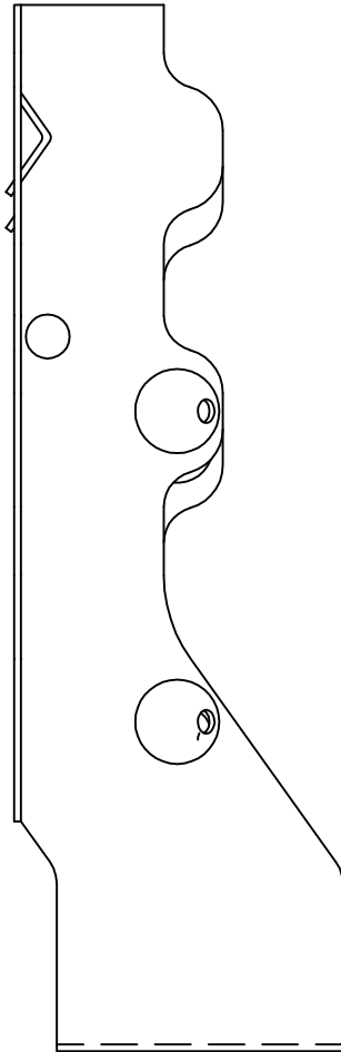
JUS28-2 - SIDE VIEW
