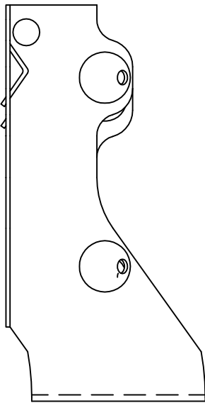
JUS26-3 - SIDE VIEW
