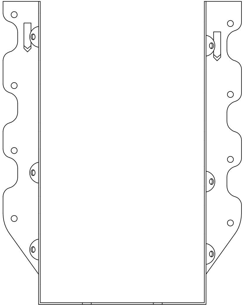
JUS210-3 - FRONT VIEW
