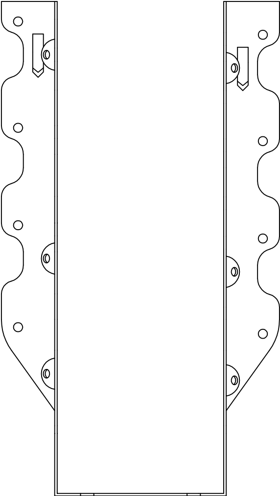
JUS210-2 - FRONT VIEW
