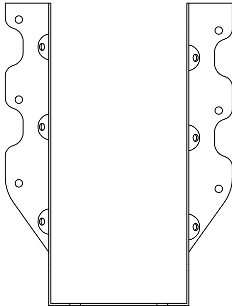
HUS28-2 - SIDE VIEW HUS28-2 - FRONT VIEW
