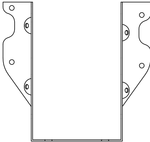
HUS26-2 - FRONT VIEW
