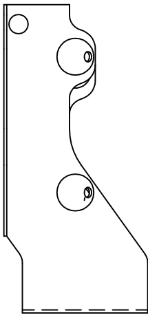
HUS26-2 - SIDE VIEW
