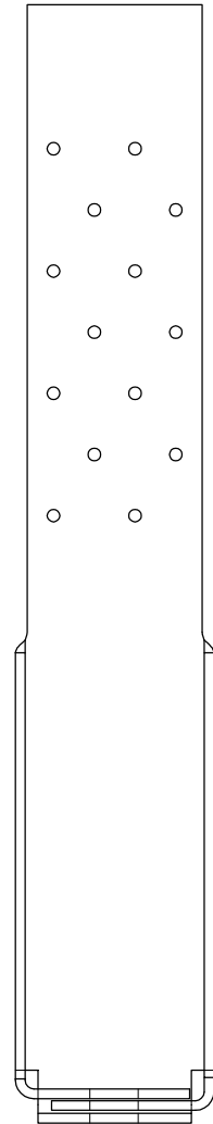
HTT14S-FRONT-VIEW
