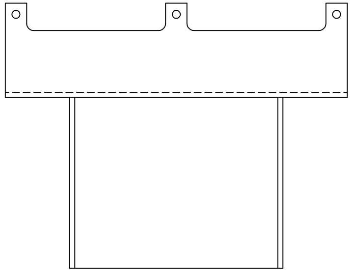
HLBH7114 - TOP VIEW
