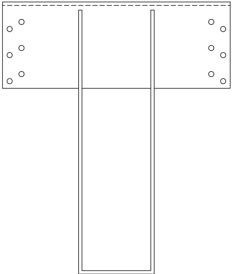
HLBH3514 - FRONT VIEW
