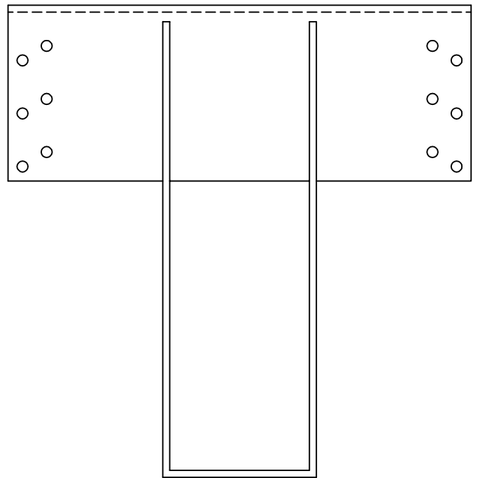
HLBH35118 - FRONT VIEW
