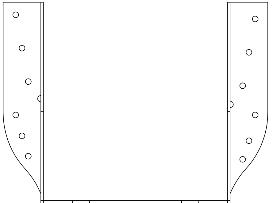
HD68 - FRONT VIEW
