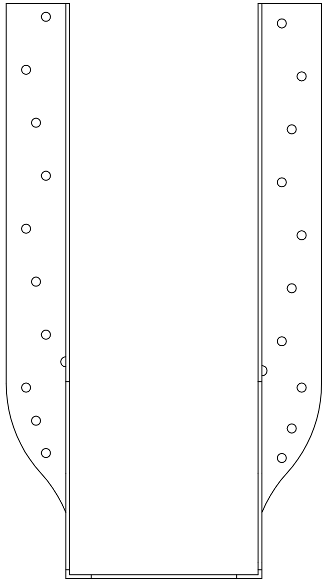
HD412 - FRONT VIEW
