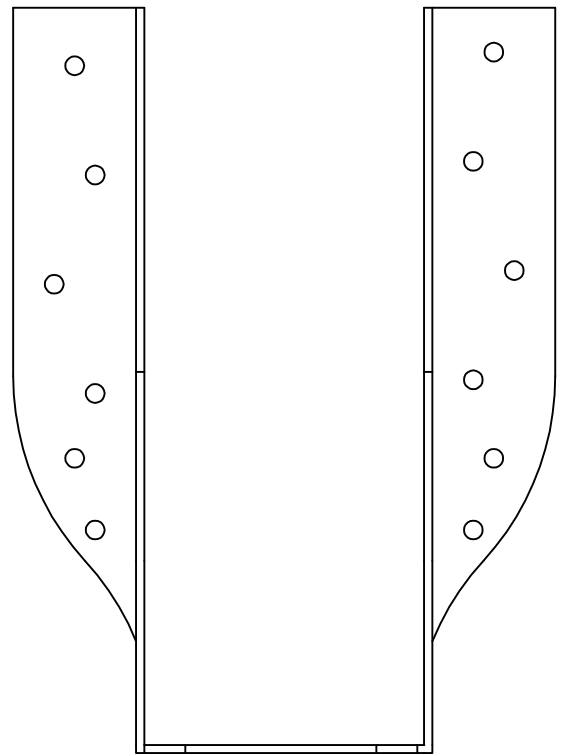
HD38 - FRONT VIEW
