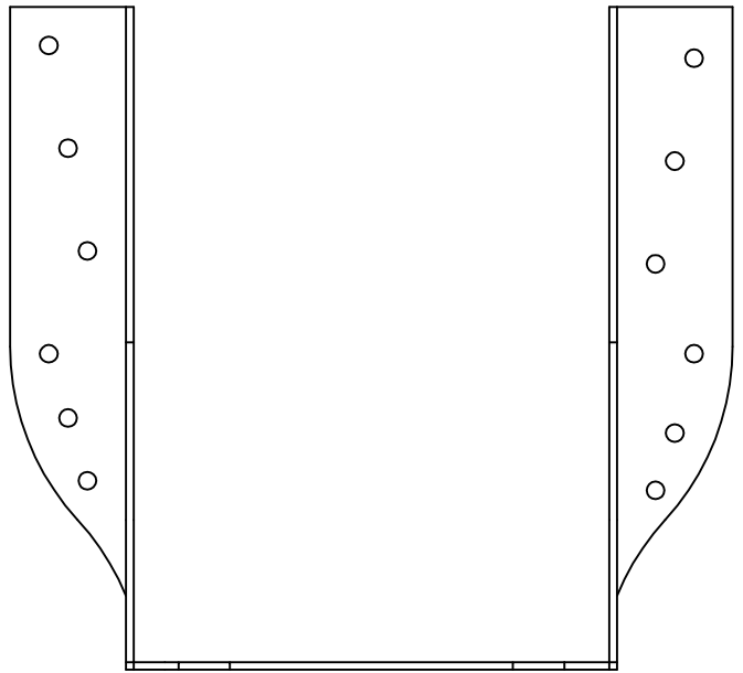
HD28-3 - FRONT VIEW
