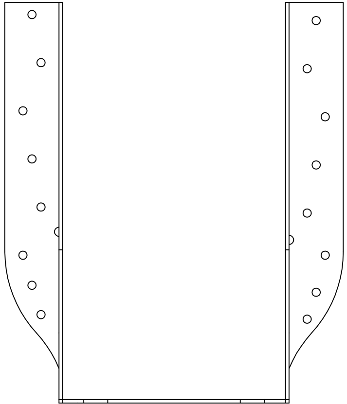
HD210-3 - FRONT VIEW
