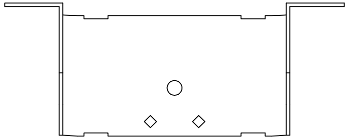
HD210-3 - TOP VIEW
