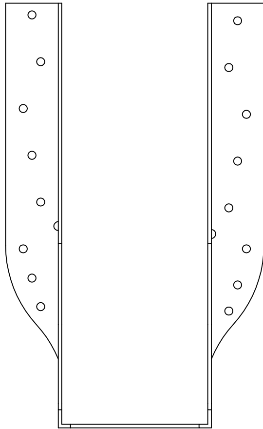
HD210-2 - FRONT VIEW
