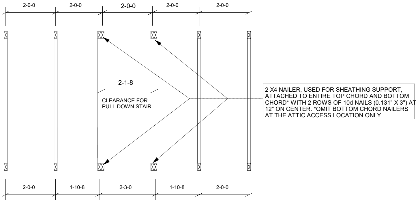
TRUSS LAYOUT DIMENSIONS TRUSSES TO BE DESIGNED AT 24" O.C.
