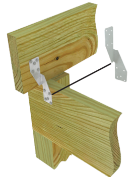
Typical RT7A installation
