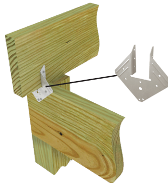
Typical RT15-TZ installation
