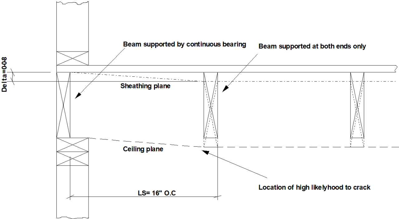
Figure 3: Differential Deflection between Beam Members
