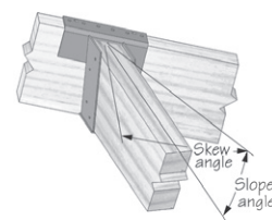
Fig. 3 - Sloped down, skewed right, low side flush shown
