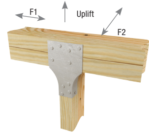
Typical SPT24 installation
