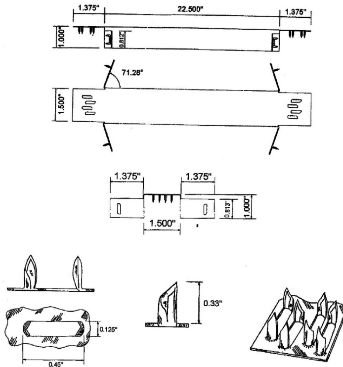
FIGURE 1—STABILIZER™
