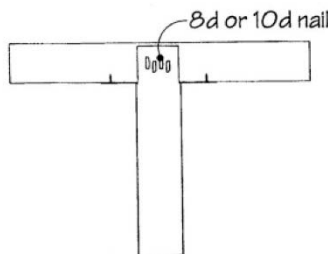
FIGURE 2—FASTENER INSTALLATION
