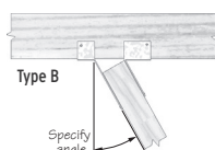
Fig. 5 - Sloped top flange, right shown
