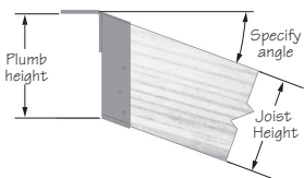
Fig. 4 - Skewed right, sloped down, top flange sloped
