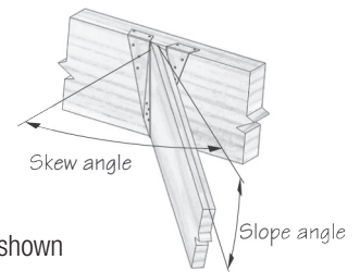
Fig. 3 - Skewed right, sloped down, low side flush shown
