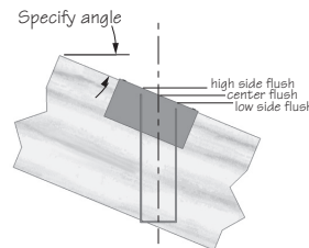
Fig. 5 - Sloped top flange, right shown
