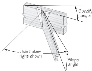
Fig. 4 - Skewed right, sloped down, top flange sloped
