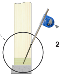
Stud to Single Bottom Plate Narrow Face (WSTS45)
