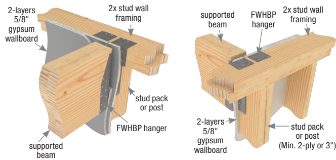
Typical FWHBP attachment to top plate/beam and stud pack/post
