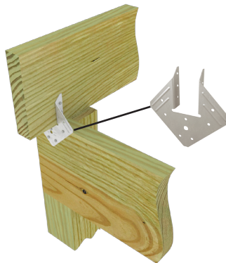
Typical RT15-TZ installation
