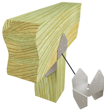
Typical C44-TZ installation
