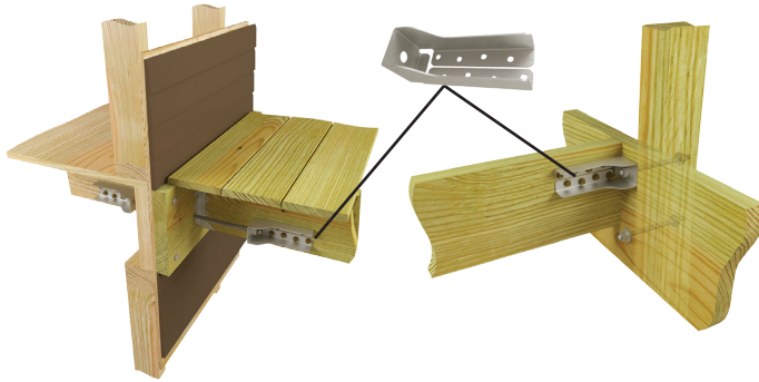
Typical DTB-TZ installations
