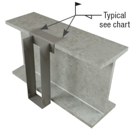
Typical top angle welded installation
