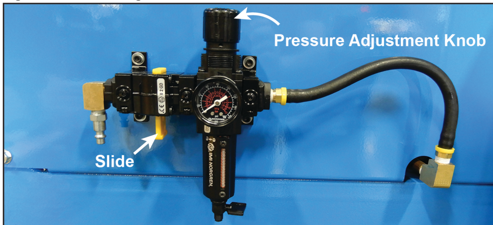
Figure 7-8: Filter / Regulator
