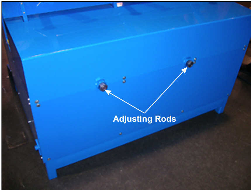
Figure 7-2: Roller Adjusting Rod Location
