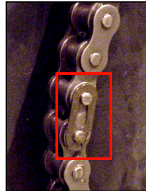
Figure 7-6: Master Link on a Chain
