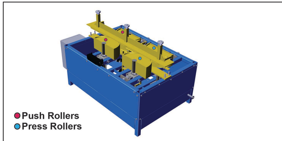
Figure 7-4: Roller Locations
